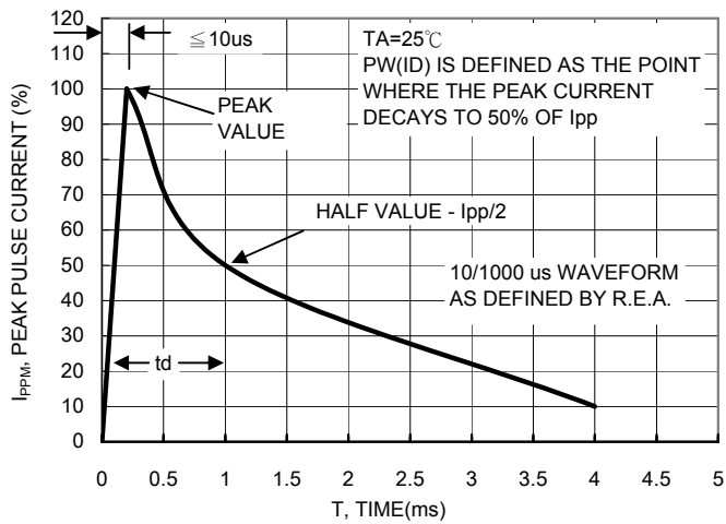
FIG. 7 PULSE WAVEFORM
