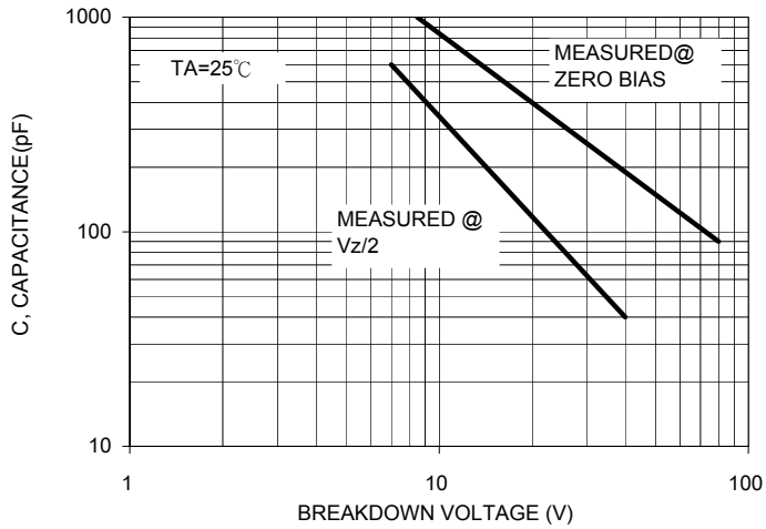
FIG.5 CAPACITANCE CURVE
