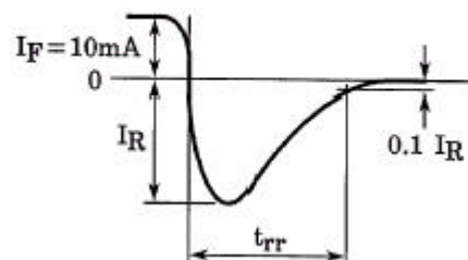
OUTPUT WAVEFORM
