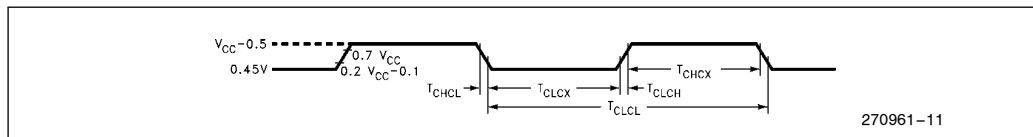
Figure 10. Clock Signal Waveform for I_{CC} Tests in Active and Idle Modes. T_{CCH} = T_{CHCL} = 5 \text{ ns}.
