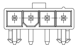
2029154-4 MATING FACE
