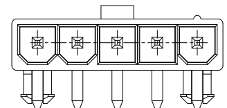
2029154-5 MATING FACE
