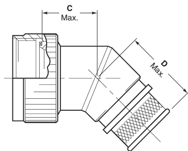
45° Adapter Code 45
