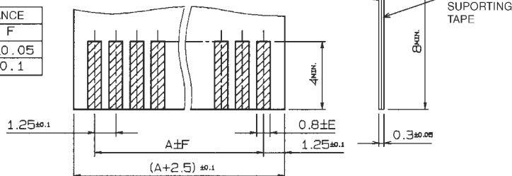
適合FPC, FFC寸法 APPLICABLE FPC/FFC
