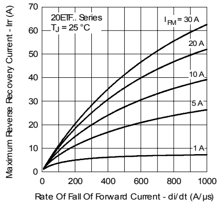
Fig. 12 - Recovery Current Characteristics, T_J = 25^\circ\text{C}
