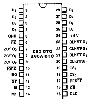
Figure 2a. 40-pin Dual-In-Line Package (DIP), Pin Assignments
