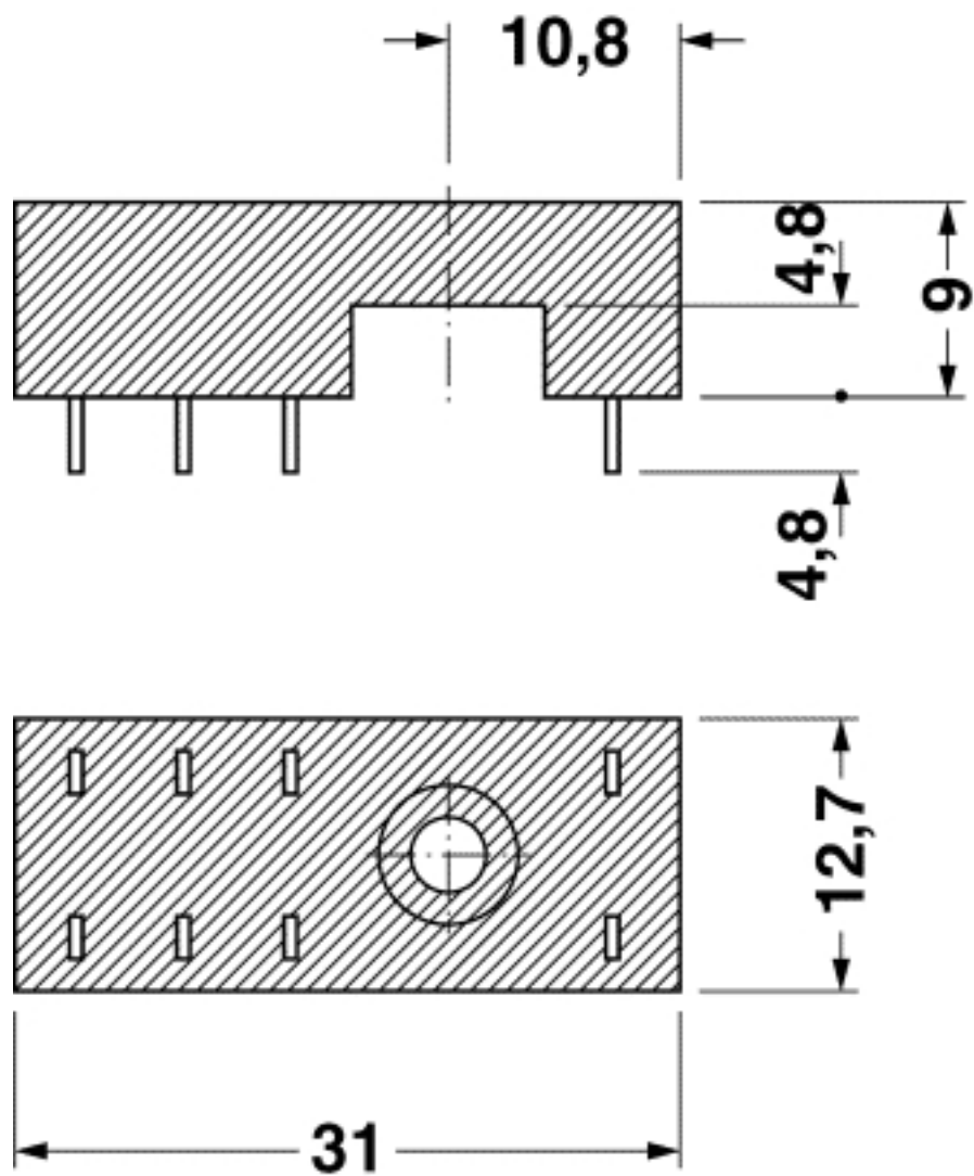
Dimensional drawing
