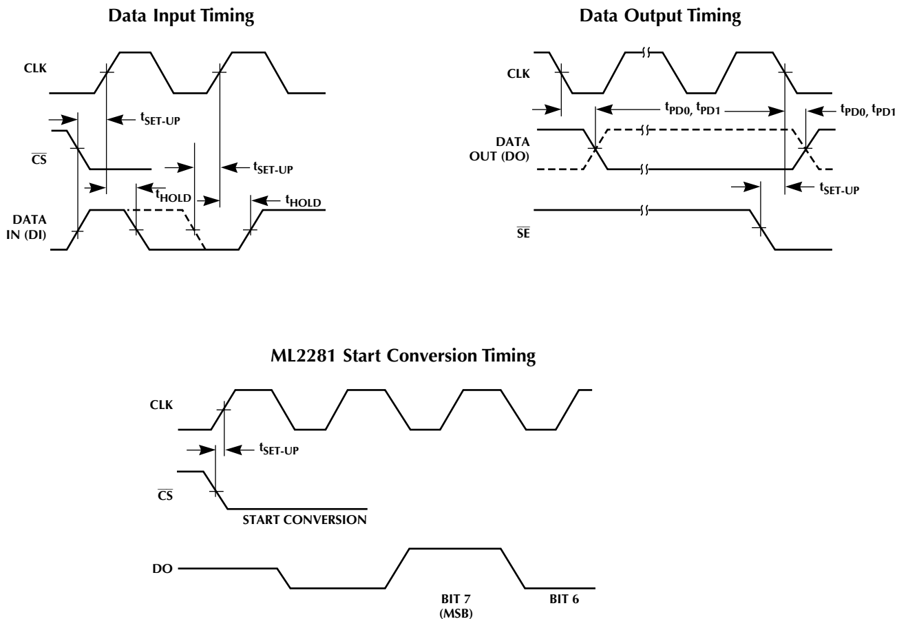
Figure 2. Timing Diagrams
