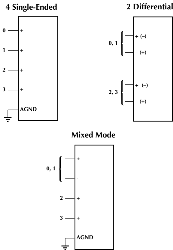
Figure 7. Analog Input Multiplexer Functional Options for ML2288
