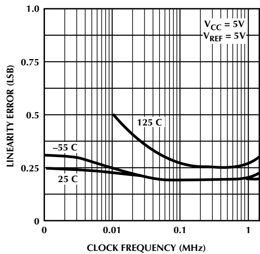
Figure 3. Linearity Error vs f_{CLK}
