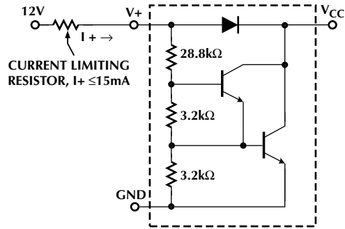
Figure 9. Shunt Regulator
