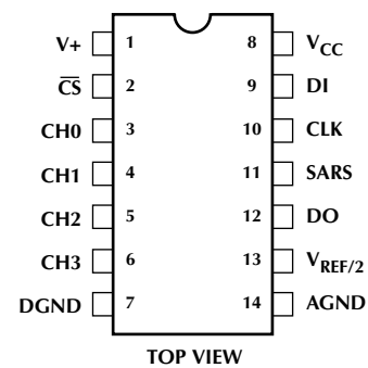
ML2283 4-Channel MUX 14-Pin PDIP
