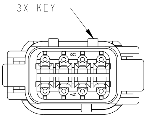
DTM06-08SC-E003 KEY -C- COLOR: GREEN
