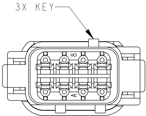
DTM06-08SA-E003 KEY -A- COLOR: GREY
