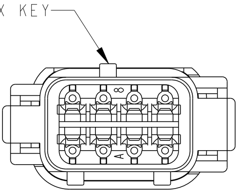
DTM06-08SD-E003 KEY -D- COLOR: BROWN
