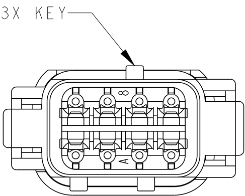
DTM06-08SB-E003 KEY -B- COLOR: BLACK
