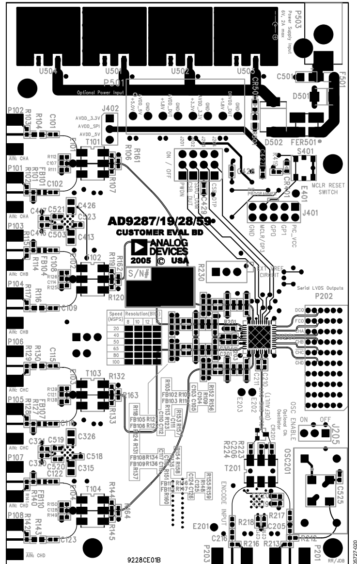
Figure 78. Evaluation Board Layout, Primary Side
