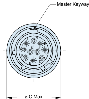
WIRE ACCOMODATION
