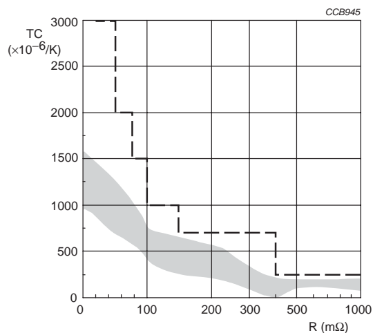
Fig.2 Typical TC as a function of resistance.
