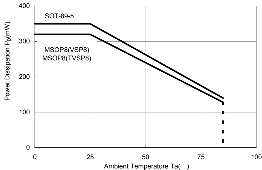
NJM2370 Power Dissipation (Topr=-40 ~ +85 ,Tj=125 )
