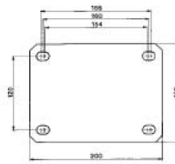
Ø 250/76-280/76
