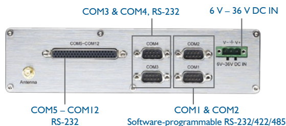
MXE-1212/232 Back Panel
