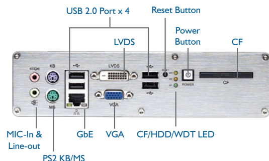
MXE-1200 Series Front Panel
