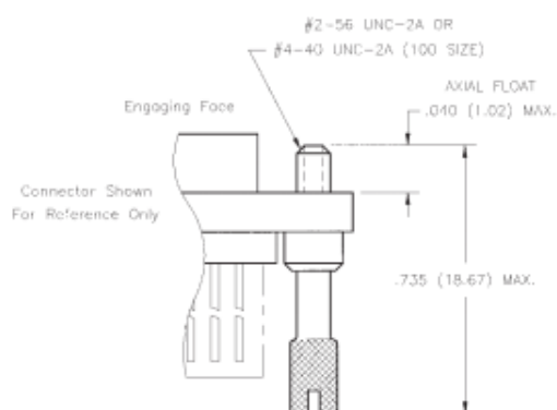
Standard Jackscrew
