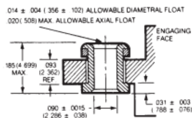
Float Mounting
