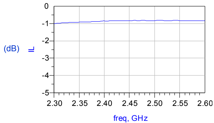
Insertion Loss
