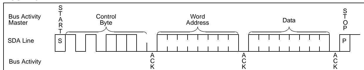
FIGURE 6-1: BYTE WRITE
