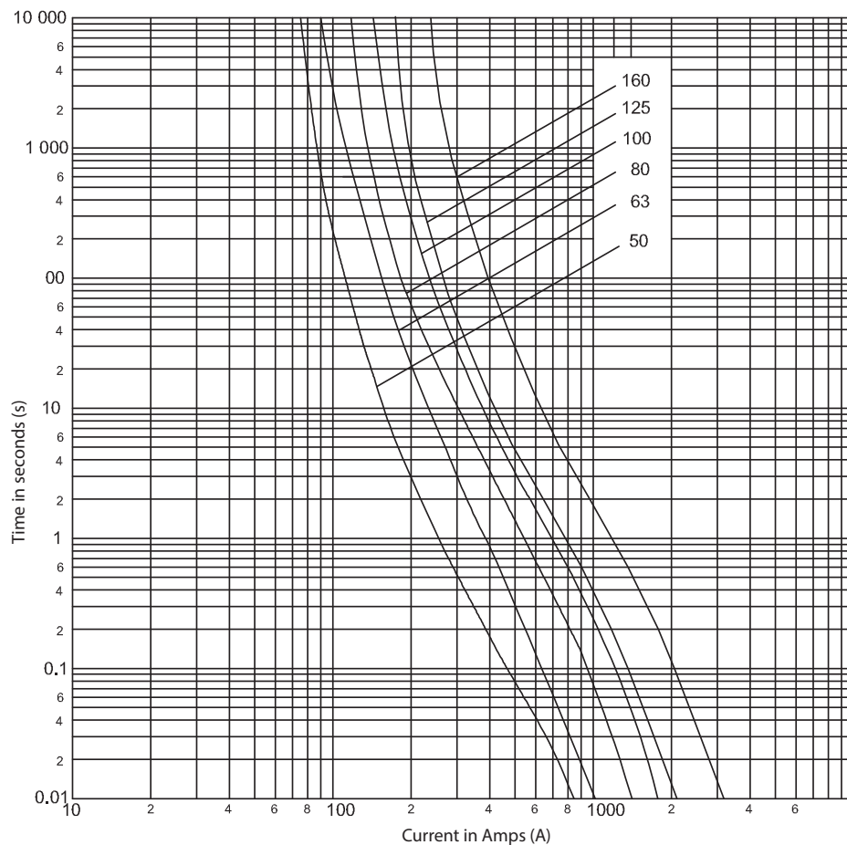
Time-current curves - NH Size 00
