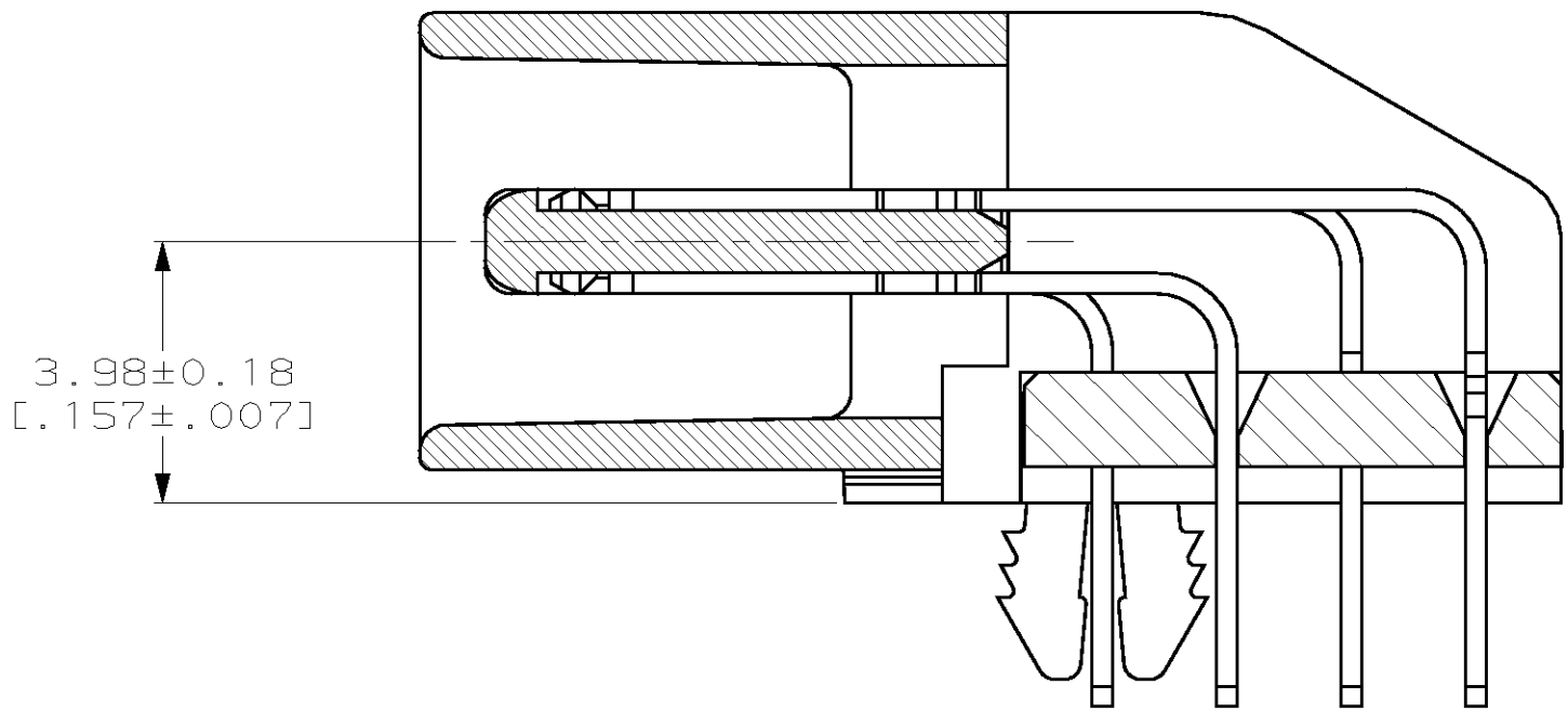
SECTION D-D SCALE 8:1
