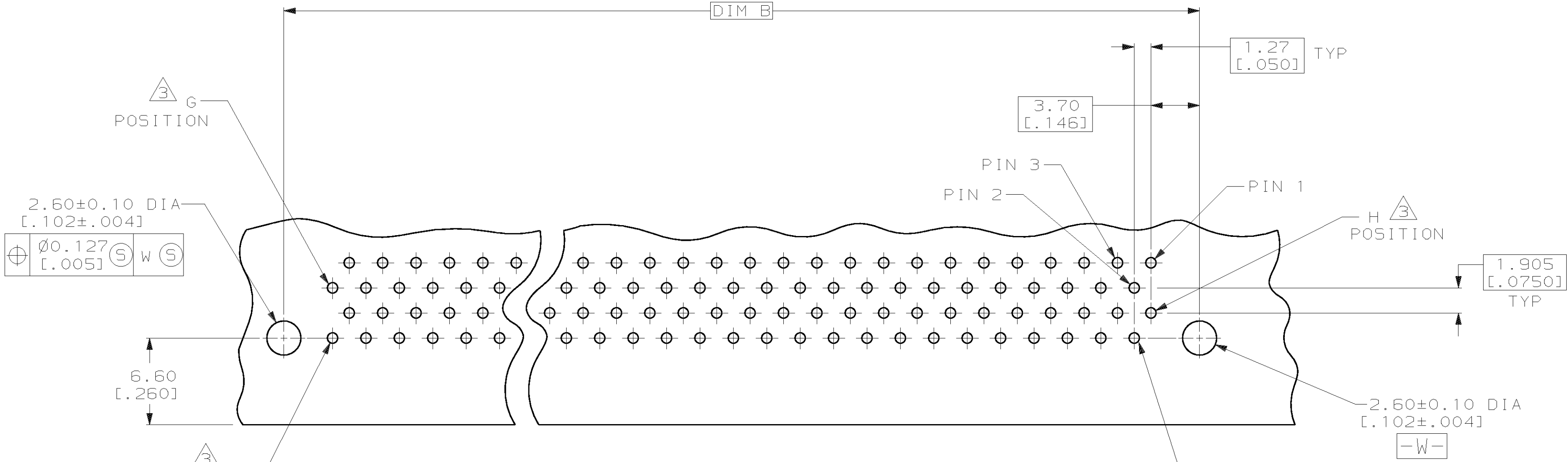
RECOMMENDED PC BOARD MOUNTING DIMENSIONS COMPONENT SIDE FOR 40, 60, 68, 80, 100, 120, 140, 160, 180 AND 200 POSITIONS ONLY
