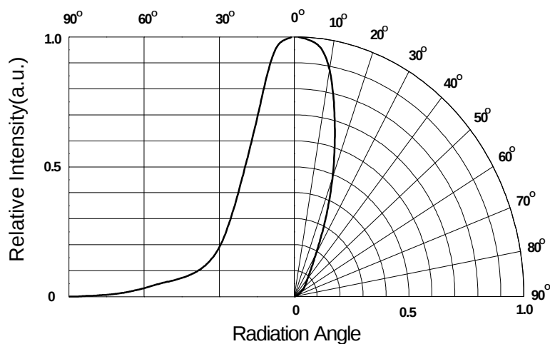
Radiation Characteristics
