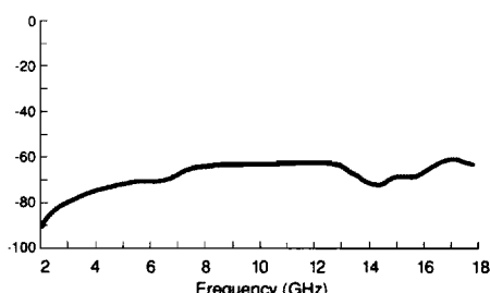
Isolation (dB)
