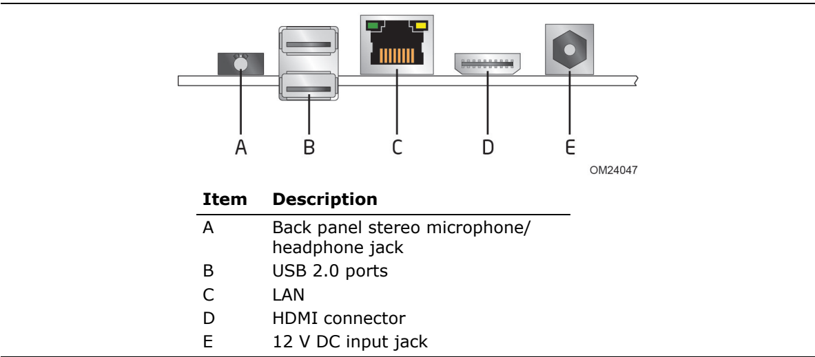
Figure 10. Back Panel Connectors
