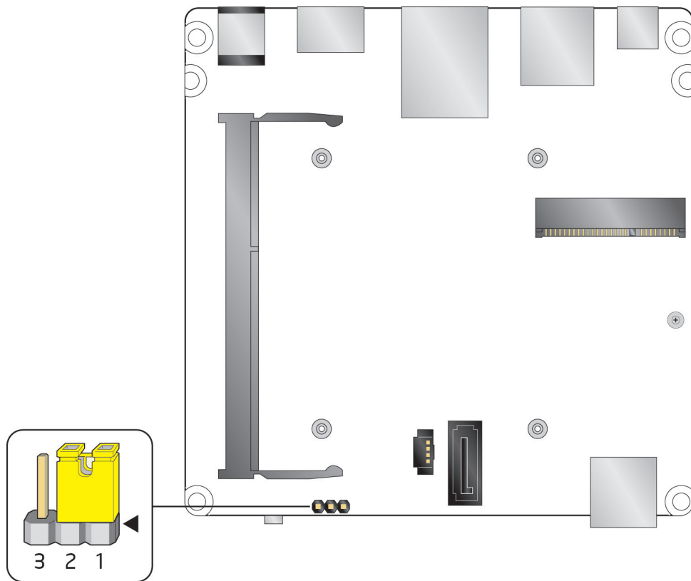
Figure 13. Location of the BIOS Security Jumper
