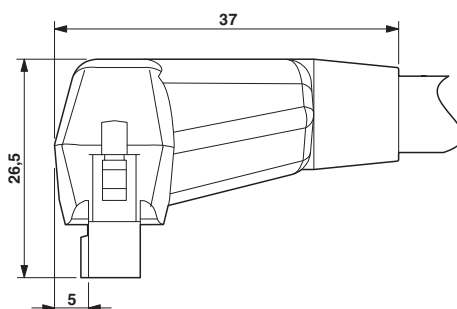
Dimensioned drawing
