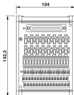
Dimensioned drawing
