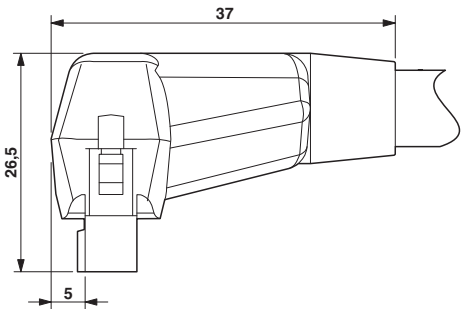
Dimensioned drawing
