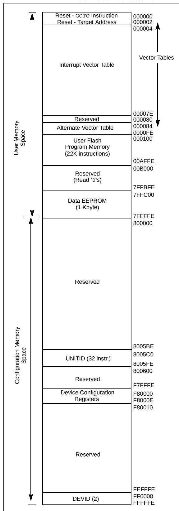
FIGURE 3-1: PROGRAM SPACE MEMORY MAP FOR dsPIC30F5015/5016
