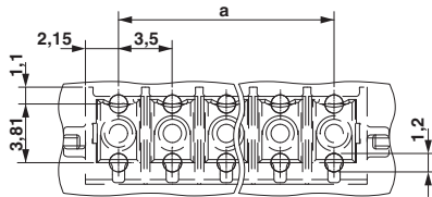
Drilling diagram
