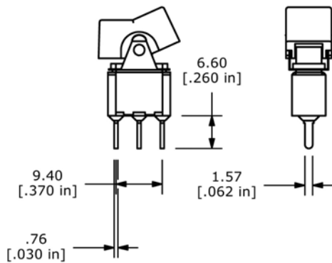
M3 Termination
