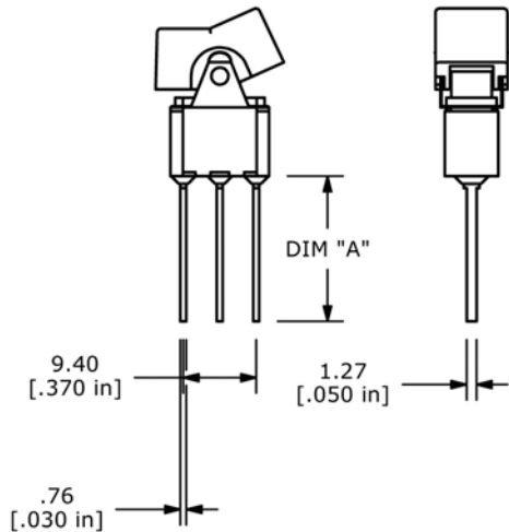
M5 Termination
