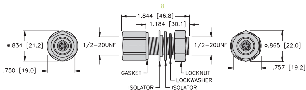
Bulkhead Feed-Thru
