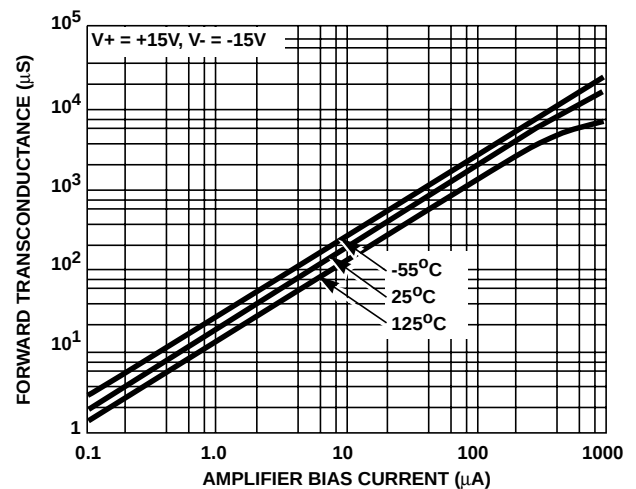
FIGURE 34. FORWARD TRANSCONDUCTANCE vs AMPLIFIER BIAS CURRENT
