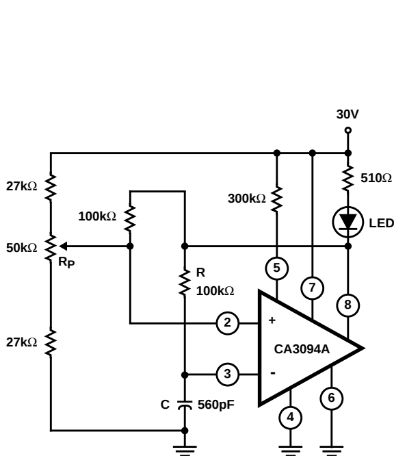
FIGURE 16. SINGLE SUPPLY ASTABLE MULTIVIBRATOR
