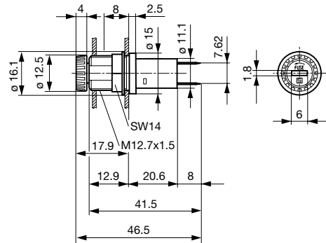
Variants Fingergrrip 3101.0125 and 3101.0325
