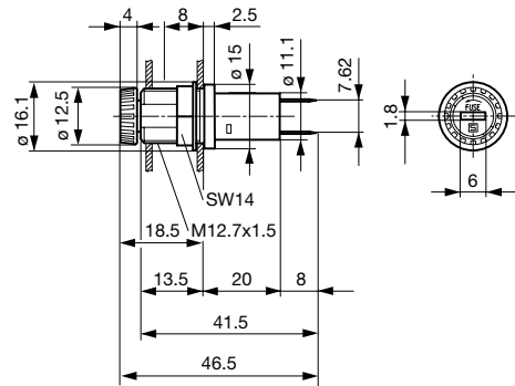
Variants Fingergrrip 3101.0025 and 3101.0225
