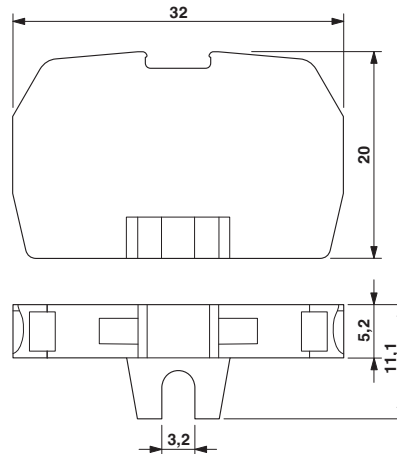
Dimensional drawing
