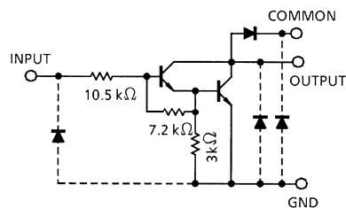
ULN2004APG/AFWG
