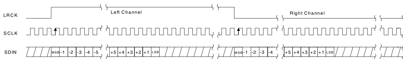
Figure 3. CS4340A Format 1 - Left Justified up to 24-Bit Data
