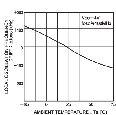
Fig. 18 Local oscillation frequency vs. ambient temperature
