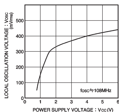
Fig. 15 Local oscillation voltage vs. power supply voltage
