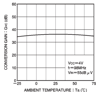
Fig. 12 Conversion gain vs. ambient temperature
