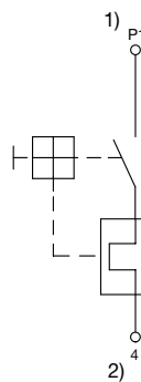
1-pole, 1 bimetal, non illuminated
