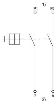
2-pole, 0 bimetal, non illuminated
