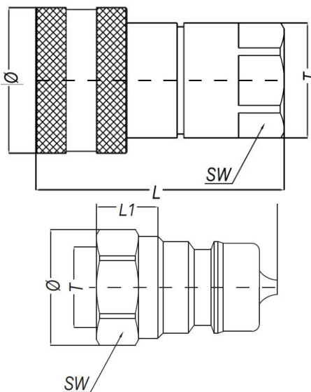
Male Self-Sealing Coupler – (e.g. 745-4700)
