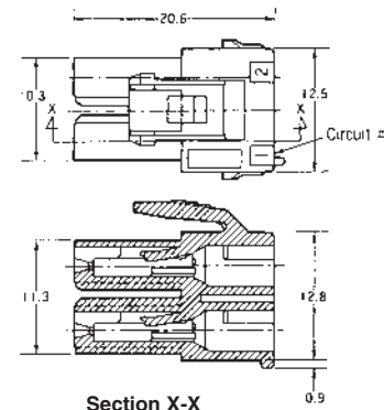
Section X-X
