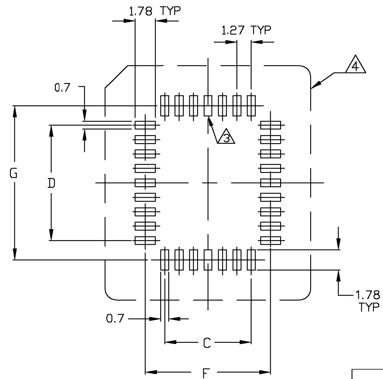
4 RECOMMENDED PCB FOOTPRINT
