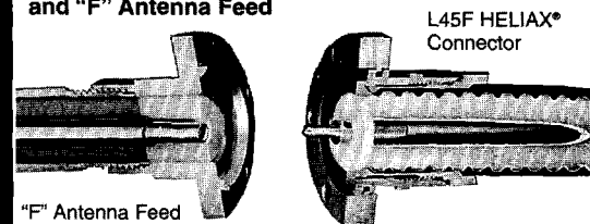
Figure 2 - "F" Flange and "F" Antenna Feed
