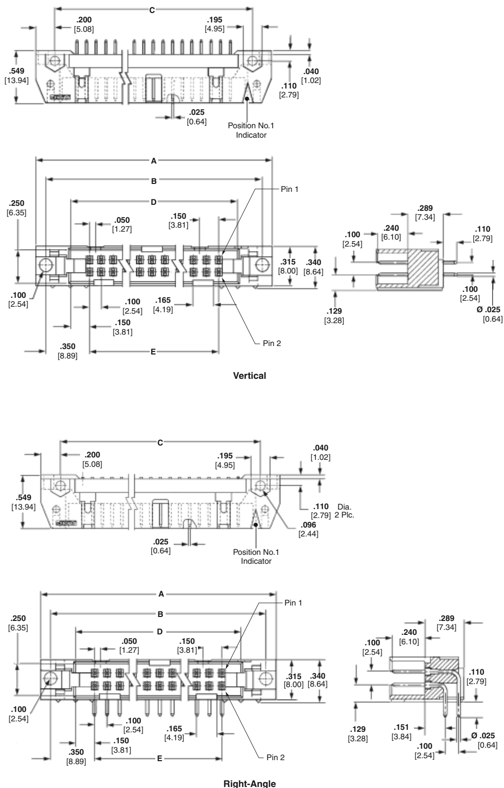
Right-Angle PCB Mount
