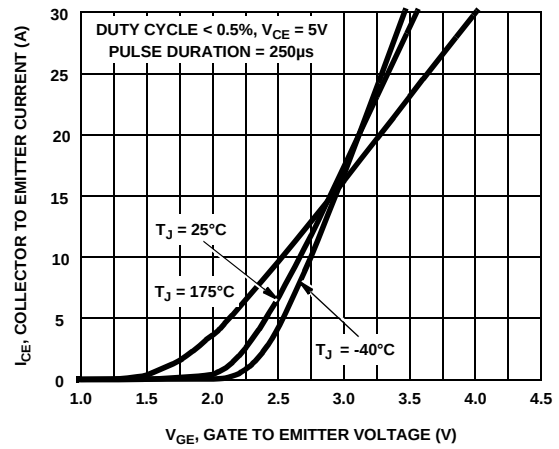
Figure 8. Transfer Characteristics
