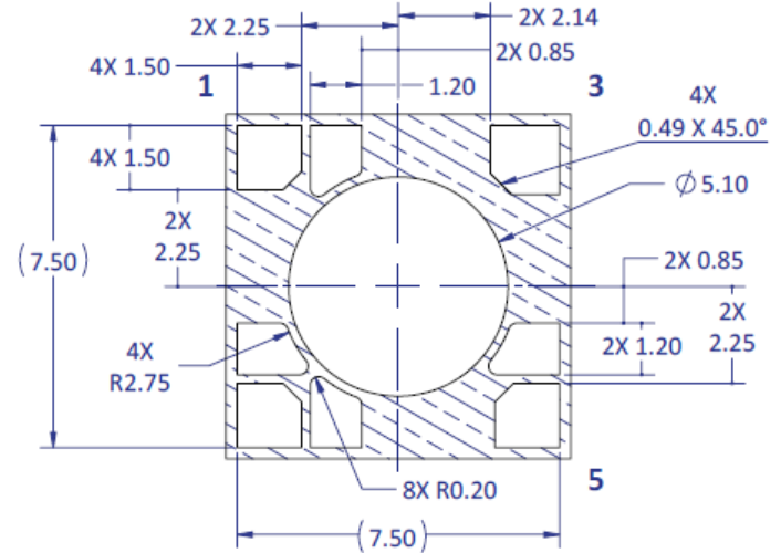
Figure 2b: Recommended solder mask opening for anode, cathode, and thermal pad for non-pedestal and pedestal design
