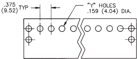
"Y" Terminal
