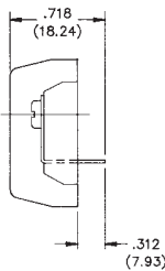
“Y” Terminals
