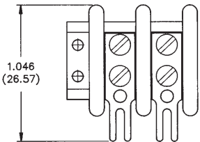
“3/4W” Terminals
