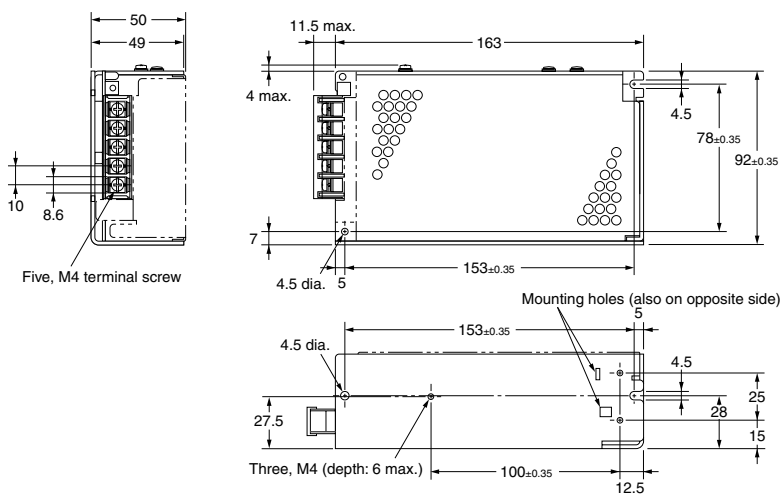
Mounting Holes
