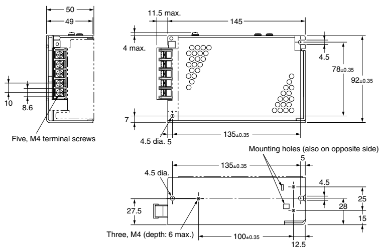
Mounting Holes
