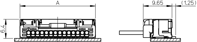
嵌合図 MATED CONNECTORES
